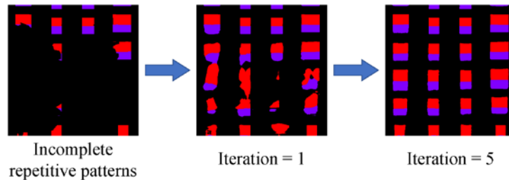
Fig. 5. Completion results of RPCNet with different iterations.
